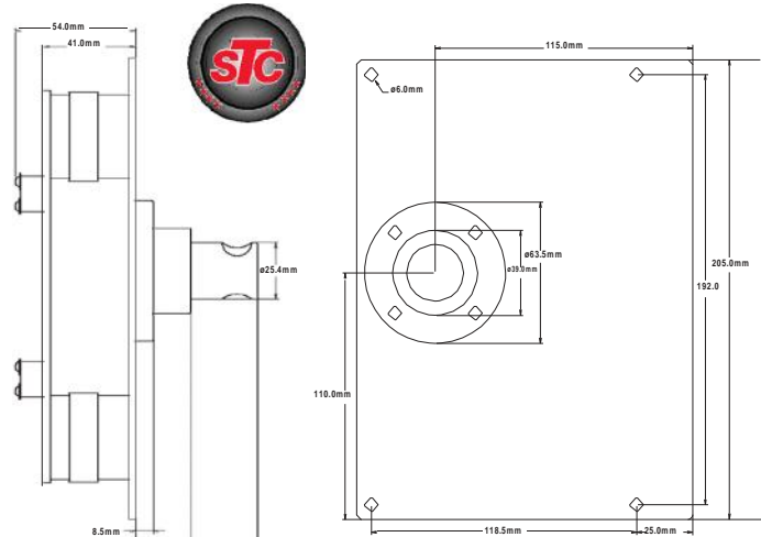
All sizes are metric in mm
